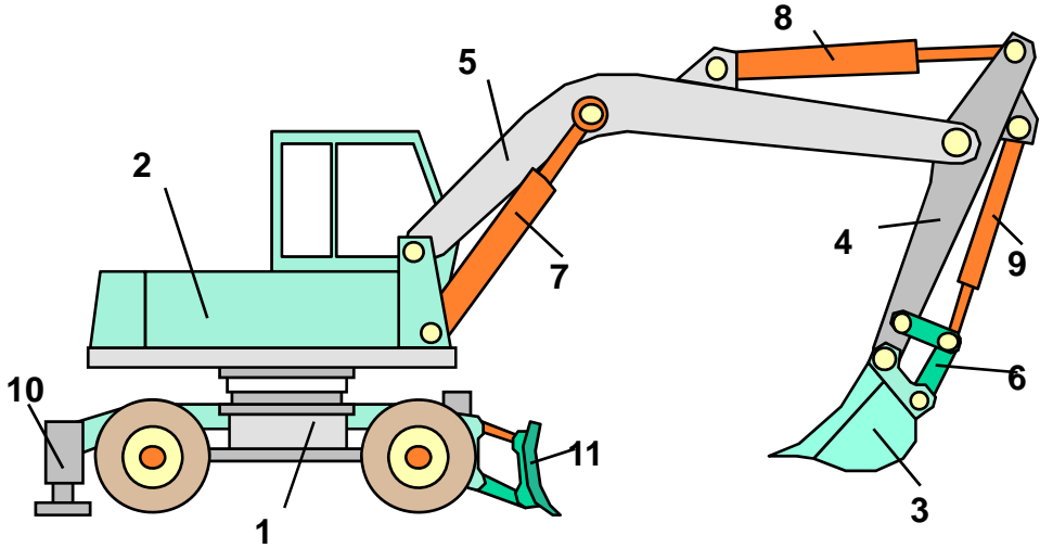
Backacter, wheel-mounted
