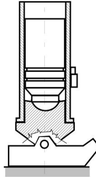
Beater-piston rammer
