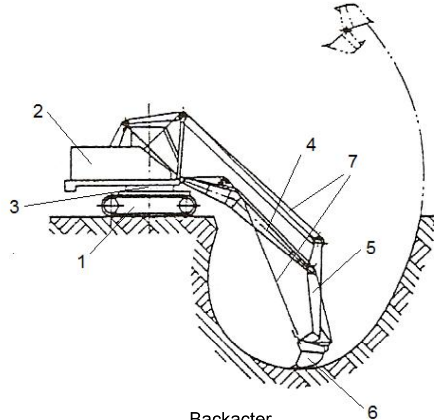
Backacter
