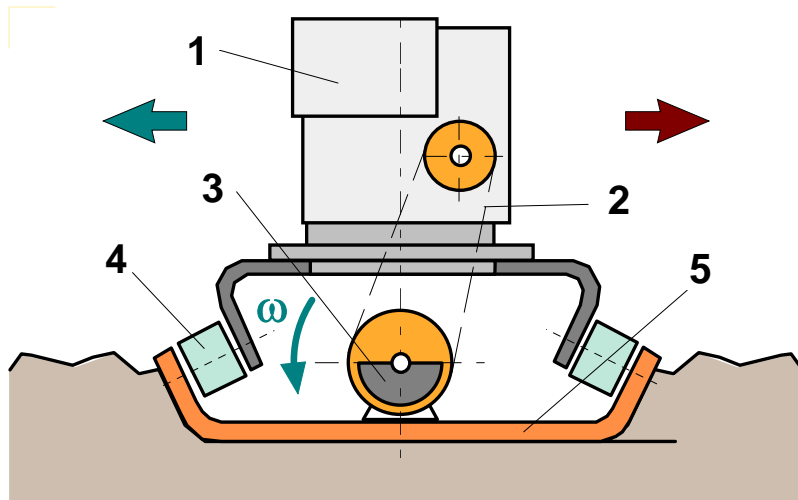
Circular excitation ( changing direction of rotation )
