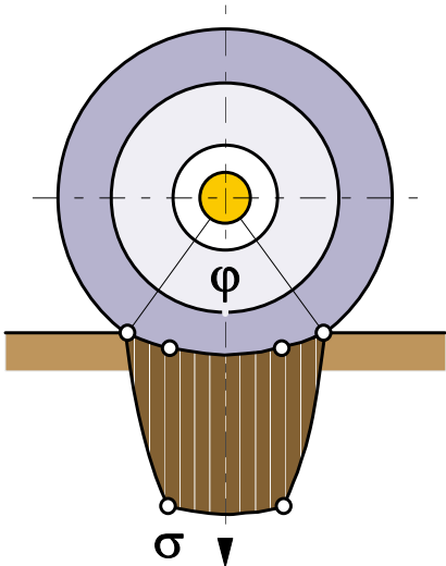
Soil compression (stress) under roller wheels
