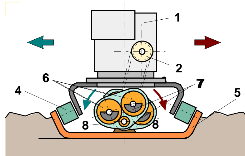
Directed excitation ( changing angle of direction )
